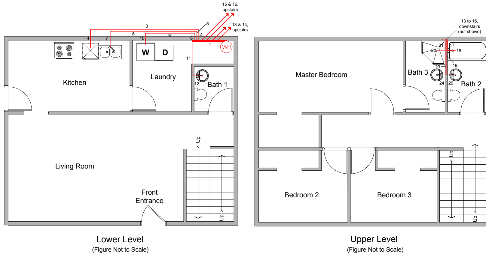
Figure 7. A Plumbing Layout Representative of a Whole-House Manifold System 20
