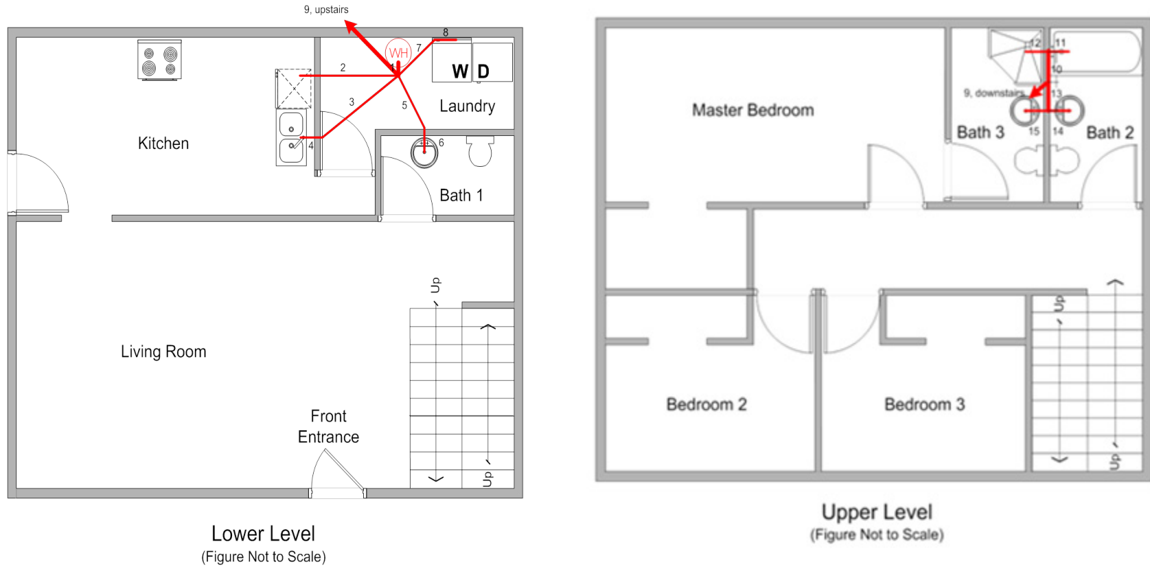
Figure 6. A Plumbing Layout Representative of a Core System 14
